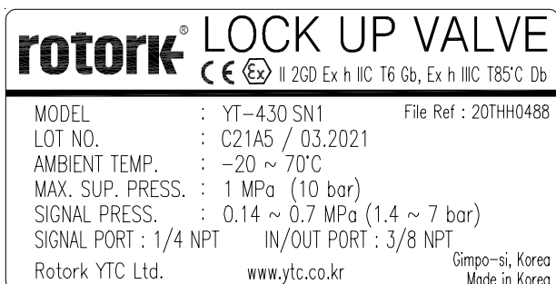
Fig. L-5: YT-430 (ATEX)
