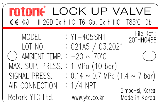
Fig. L-3: YT-405 (ATEX)
