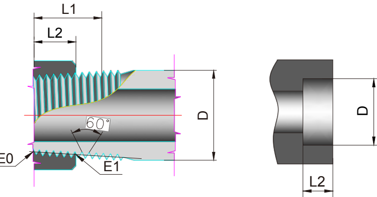
PIPE THREADS, GENERAL PURPOSE ASME B1.20.1.
