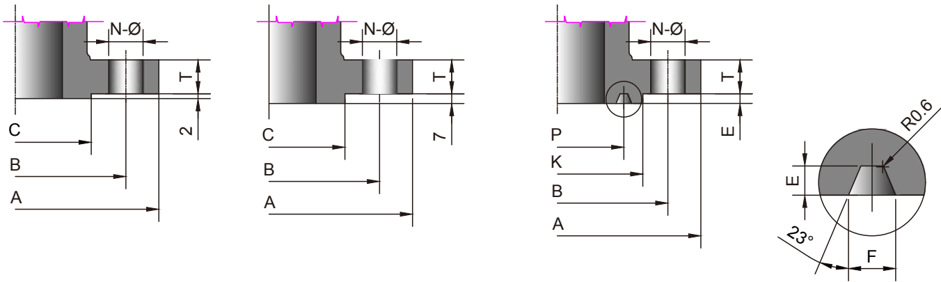
PIPE FLANGES END ASME B16.5.
