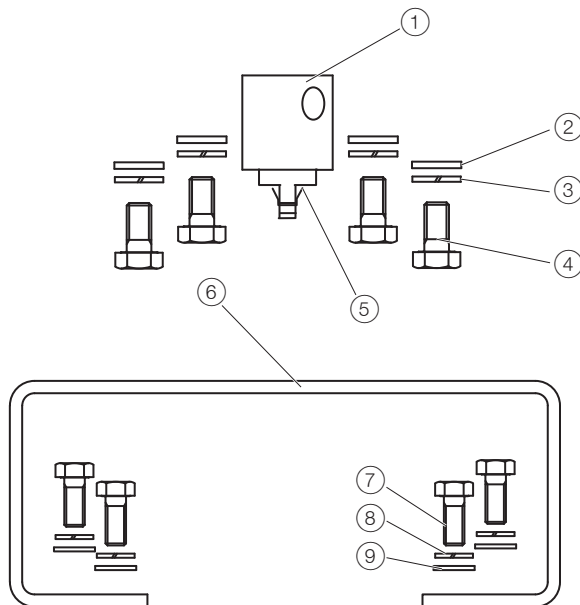
Figure 13: Components of attachment kit
