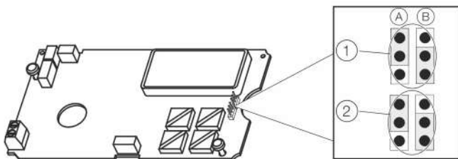
Figure 24: TZIDC-120 jumpers
