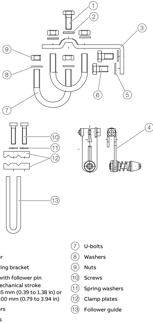
Figure 5: Attachment kit
