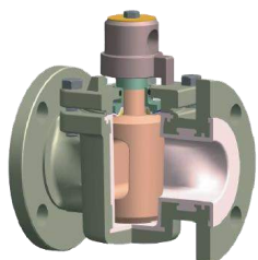
Lined Plug Valve
