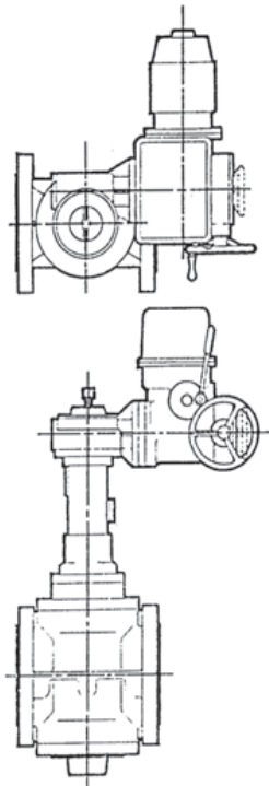
STYLE "B" MOTOR OPERATOR MOUNTED AT RIGHT ANGLE TO PIPE LINE
