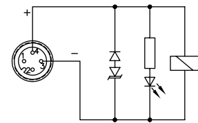
Electrical schematic
