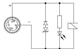
Electrical schematic
