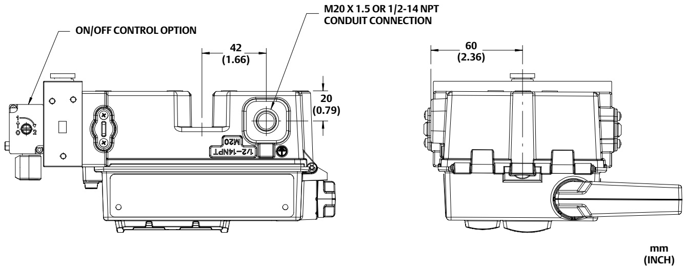
Figure 3. Dimensions—External Power Option
