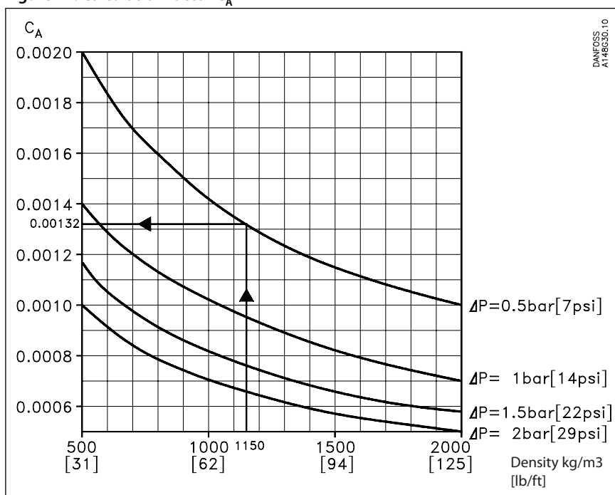
Figure 13: Flow rate diagram
