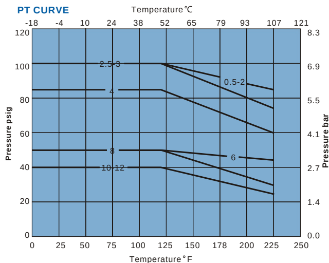
PT CURVE
