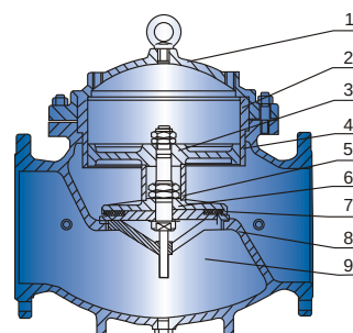
FIG.2-Piston type
