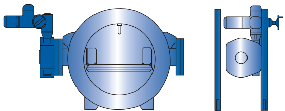
3. Worm gear unit + Electric actuator
