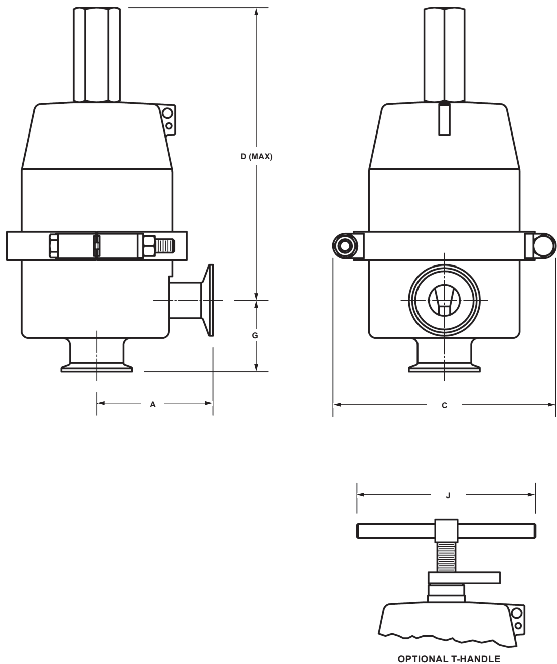
Figure 5. Dimensions
