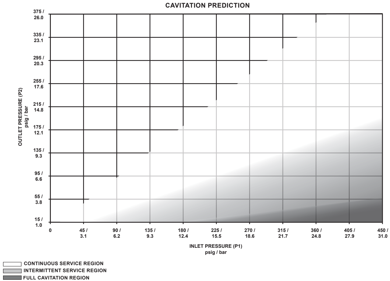
Figure 4. Cavitation Sizing for Water
