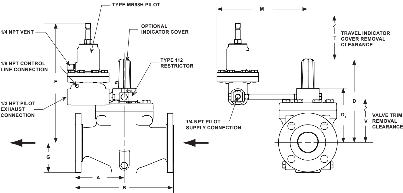
Figure 5. Type LR128 Dimensions Schematic
