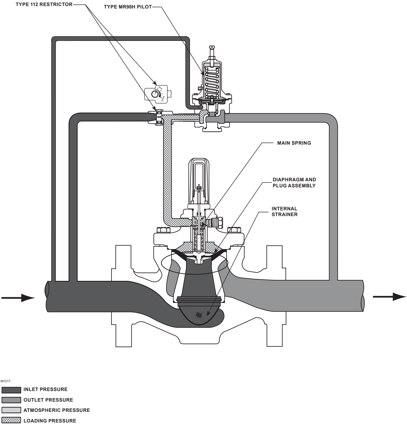
TYPE LR128 WITH TYPE MR98H PILOT AND TYPE 112 RESTRICTOR
