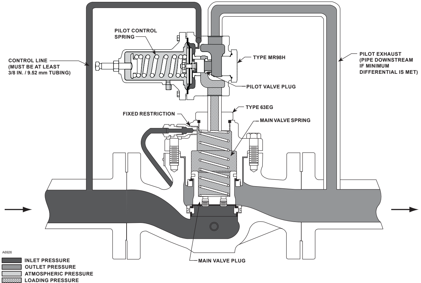
Figure 2. Operational Schematic
