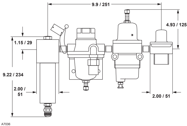
TYPE H120 RELIEF VALVE NOT SHOWN
