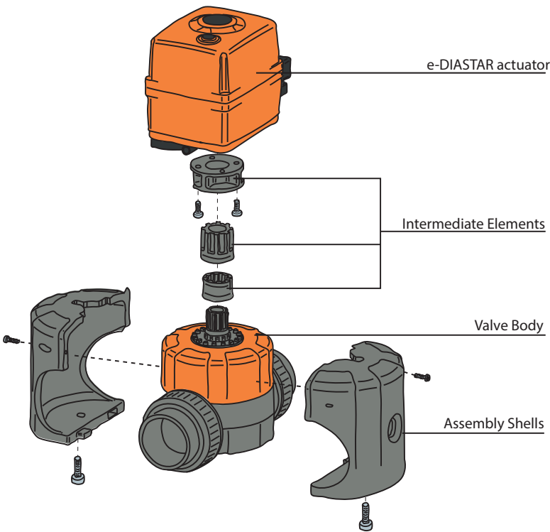
Components by Valve Type
