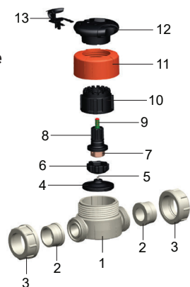
Diaphragm Valve
