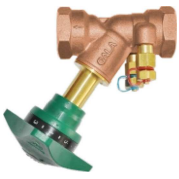
Fixed Orifice Double Regulating Valve Fig.1209-BT/BTM Standard: BS 7350 Size: DN15~DN80
