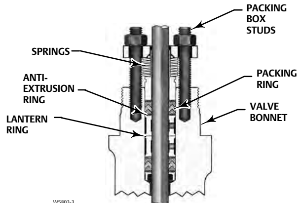
W5803-3 TYPICAL ENVIRO-SEAL PACKING SYSTEM WITH PTFE PACKING
