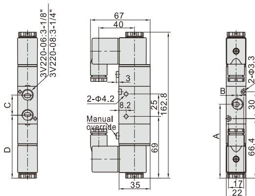
3V220(Terminal)
