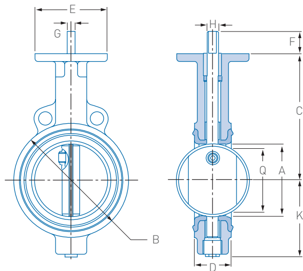
FIGURE 221 DIMENSIONS (inches)
