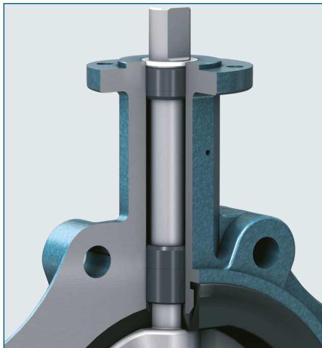
Safety seal acc. to TA-Luft/ VDI 2440, RWTÜV
