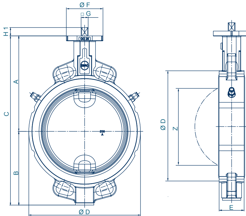
Z 011-A Inflas® with bare shaft end according to EN ISO 5211
