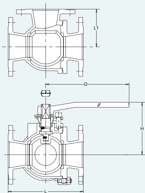
150UTR2L(M) (L-port, 2-seated) 150UTR2TM (T-port, 2-seated)
