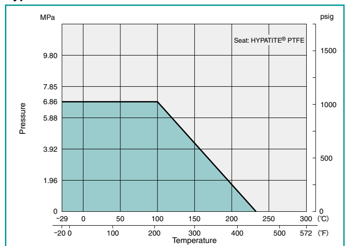
Type 1000: SC3TZ/U3TZ Series
