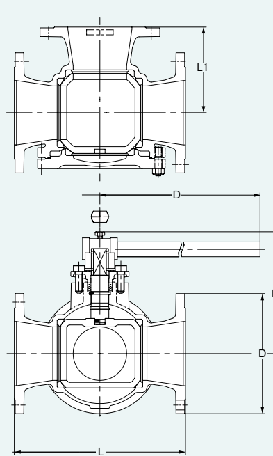
(G-)150UTR4LA(M) (L-port, 4-seated) (G-)150UTR4TA(M) (T-port, 4-seated)
