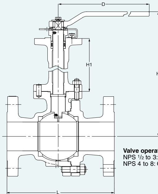
Dimensions of 300UTDZXL(M)
