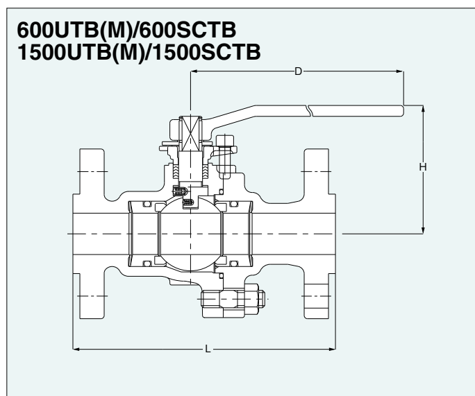
Dimensions of 600UTB(M), 600SCTB
