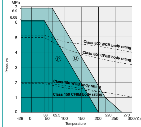
150/300UTAZ(M)/SCTAZM : NPS 8, 10
