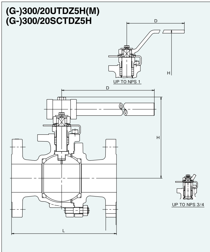
Dimensions of 300UTDZ5H(M), 300SCTDZ5H
