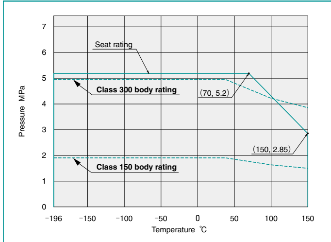
150/300UTAZL(M): NPS 4, 6
