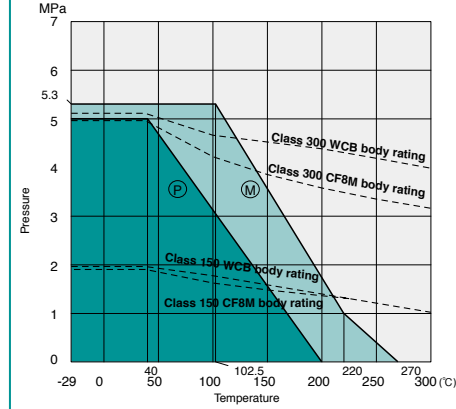
150/300UTAZ(M)/SCTAZM : NPS 1½ to 3
