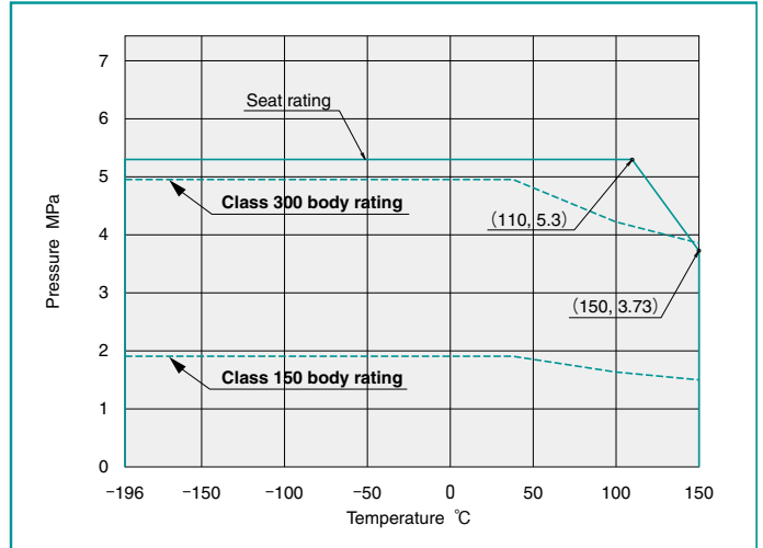
150/300UTAZL(M): NPS 3
