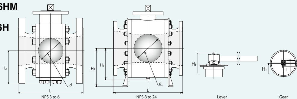
Dimensions of T60M/(G-)300UF3TCR6HM, T60M/(G-)300SF3TCR6H
