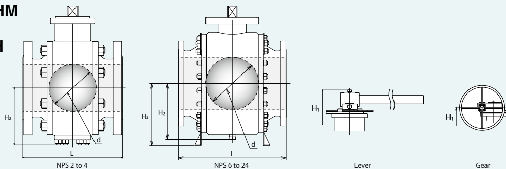
Dimensions of T60M/(G-)300UF3TC6HM, T60M/(G-)300SF3TC6H
