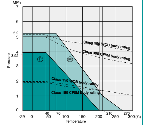
150/300UTAZ(M)/SCTAZM : NPS 4, 6
