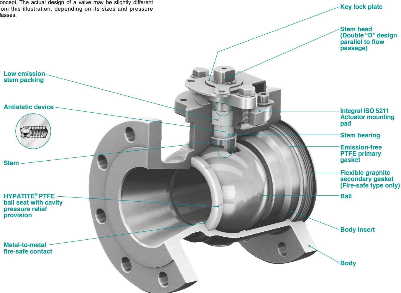
150SCTAZ Size 1 1/2
