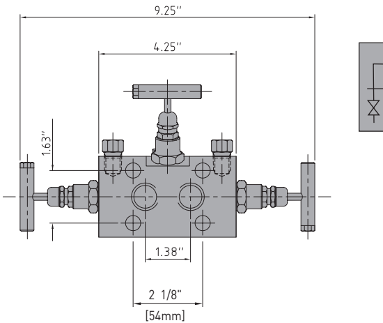
Direct mounting pipe to flange manifold, with vent ports.
