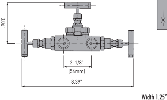
Remote mounting pipe to pipe, with vent ports.
