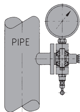
VERTICAL PIPING PRESSURE MEASUREMENT
