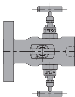
FLANGE TO FLANGE – ONE BORE – THREE STANDARD MATERIALS
