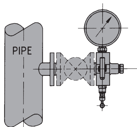
VERTICAL PIPING PRESSURE MEASUREMENT
