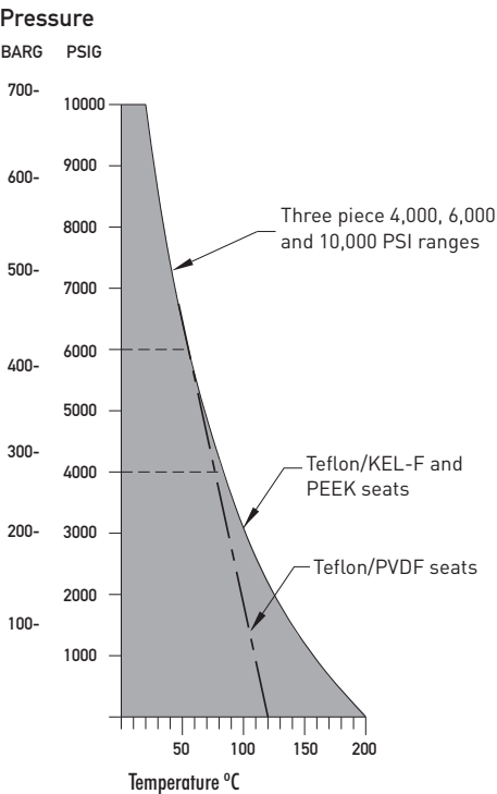
BALL VALVE PRESSURE VS TEMPERATURE CURVE
