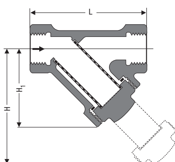
Y-type strainer with screwed connections series 330 GSF 335, PN 40, CuZn39Pb3
