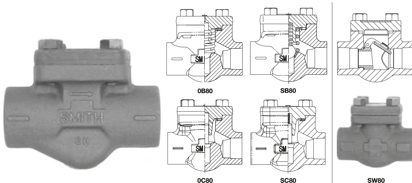
OB80 CLASS 800 BOLTED CAP BALL TYPE CHECK VALVE - THREADED or SOCKET WELD - INCHES (MM)
