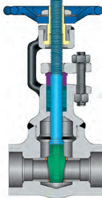
WELDED BONNET 2054W – Class 800 3054W – Class 1500
