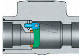
COVERLESS SWING CHECK
