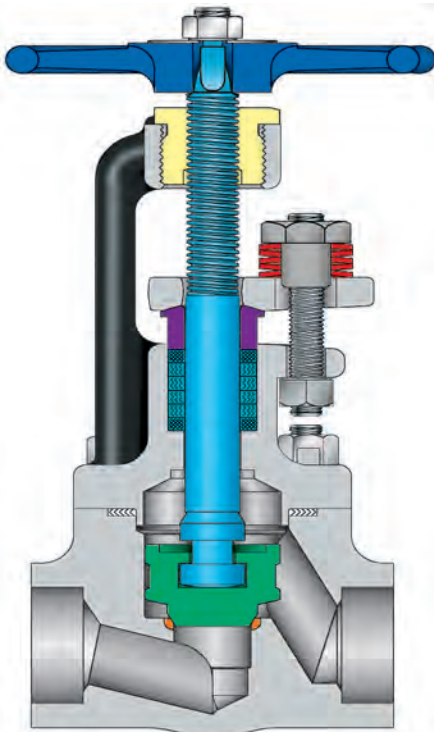
GLOBE VALVE
