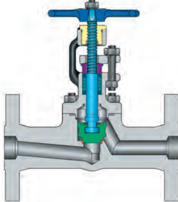
FLANGED BOLTED BONNET 0074B – Class 150 2074B – Class 600 1074B – Class 300 3074B – Class 1500
