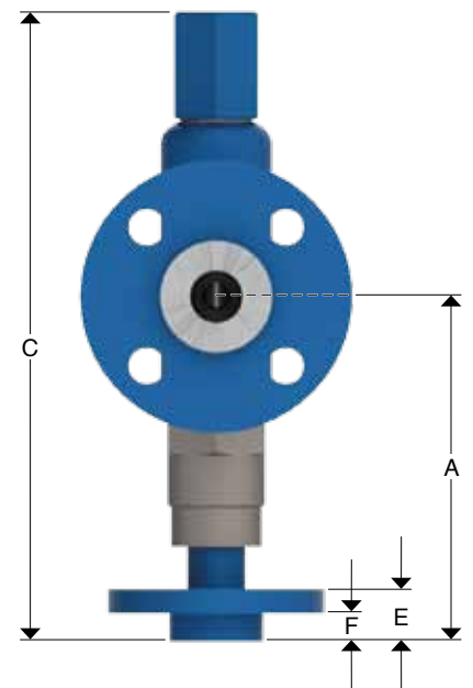
1S20 Flanged Ends (Front)
