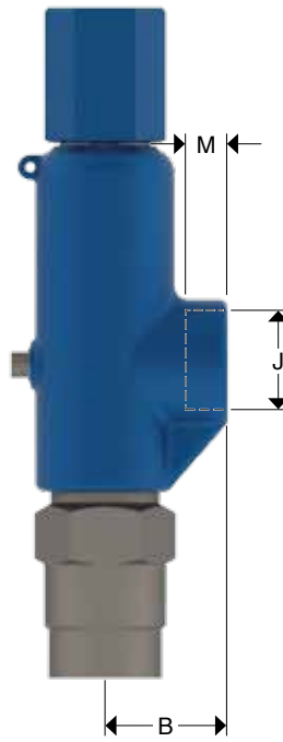
1S20 Socket Weld Ends (Side)
