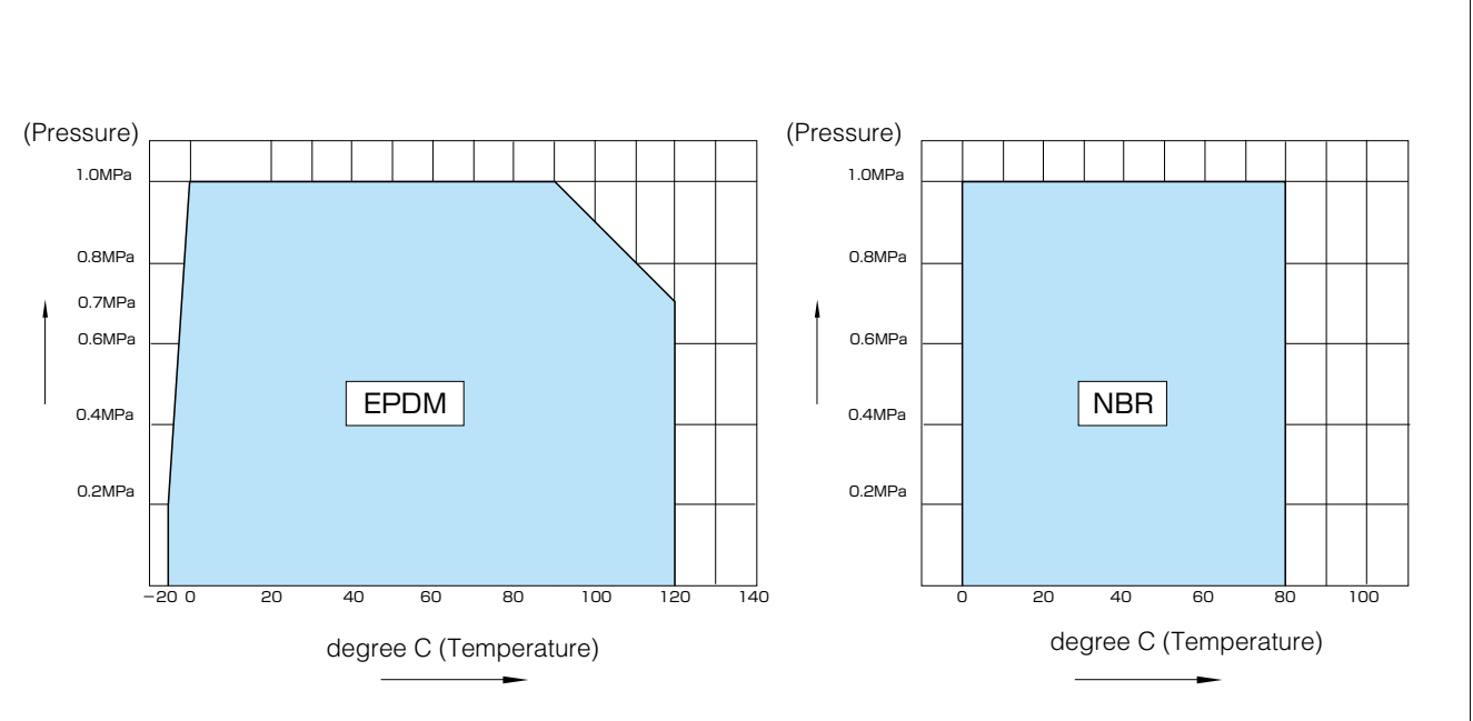
700E / 700K / 700S Pressure-Temperature Rating
