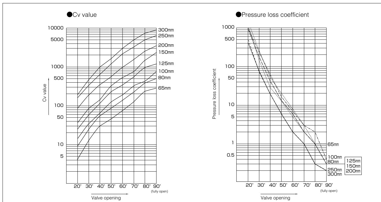
846T Cv value/pressure loss coefficient
