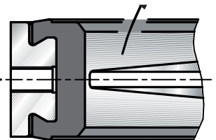
Valve opens without friction when the seat is unloaded
