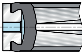
Valve closed seat ring pneumatically preloaded and bubble-tight
